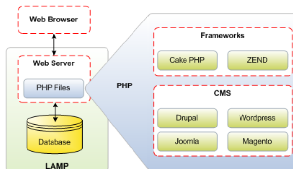
Fig 2. LAMP architecture
