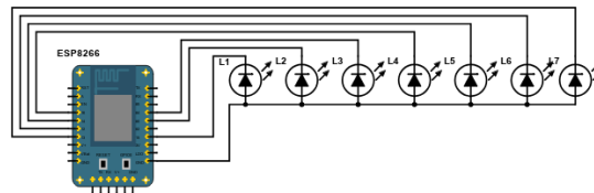
Fig. 5: Circuit Diagram for Experiment 1
