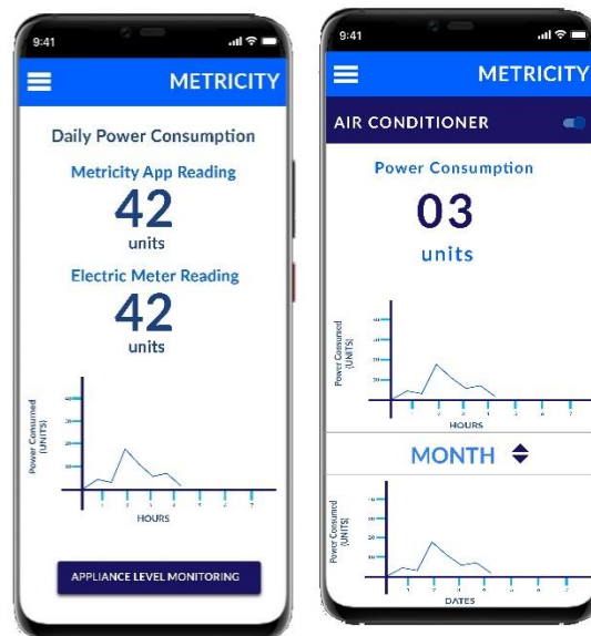
Fig. 1: Interface of the Proposed Solution
