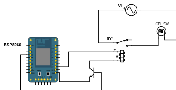
Fig. 6: Circuit Diagram for Experiment 2
