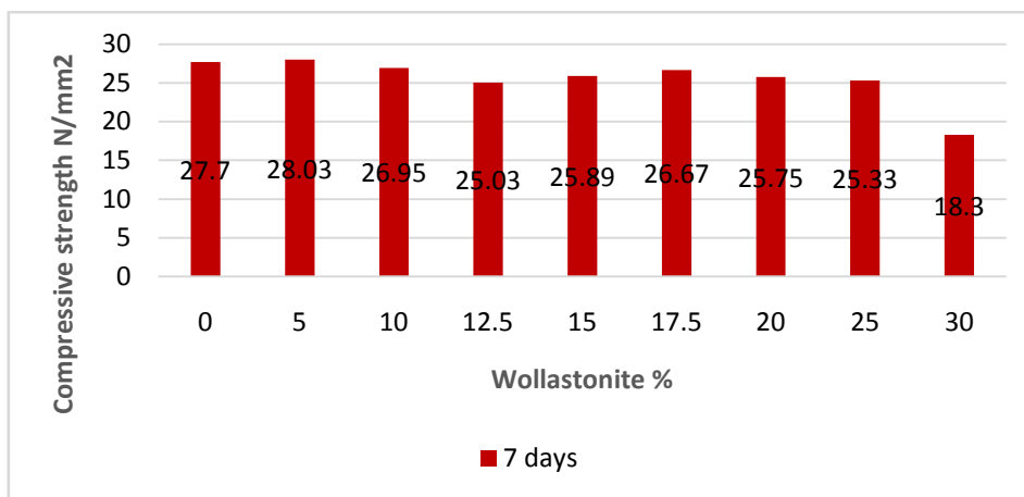
Figure 2. 7 days Compressive Strength of Concrete
