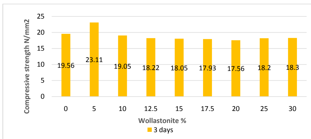
Figure 1. 3 days Compressive Strength
