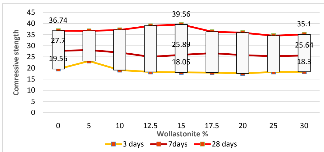
Figure 4. Combined Compressive Strength of Concrete
