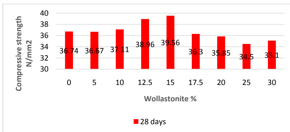
Figure 3. 28 days Compressive Strength of Concrete
